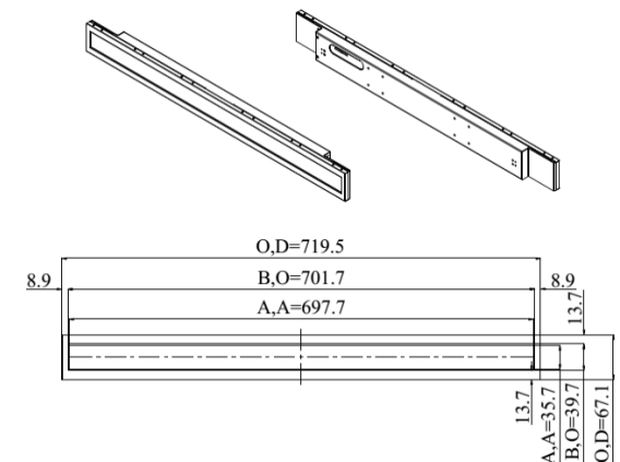
Outline Dimensions
